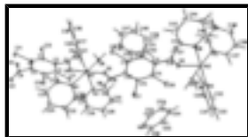
Fig. 1. The asymmetric unit of the title complex showing 30% probability displacement ellipsoids and the atom-numbering scheme.
